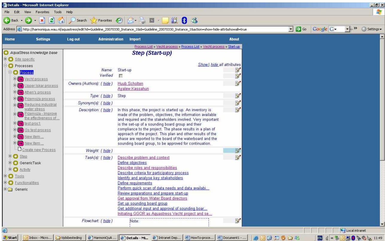
Figure 6. Main panel to edit the AQS-KB item property of the type step.
